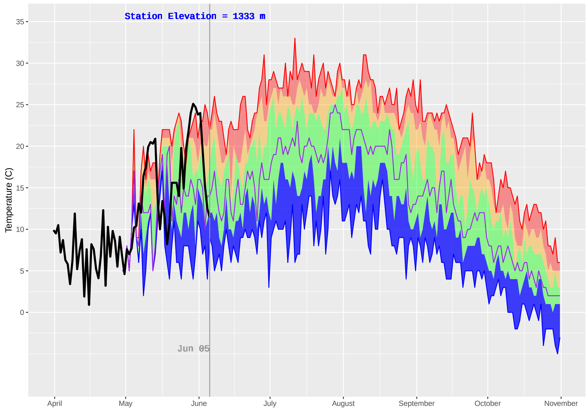
GOLDSTREAM 2 (919) : Historical (2005–2018) and Current (2019) Daily Temperature
