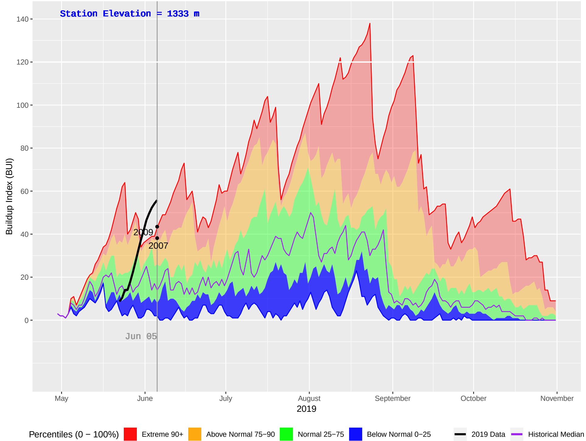
GOLDSTREAM 2 (919) : Historical (2005–2018), Current (2019) Daily Buildup Index (BUI)
