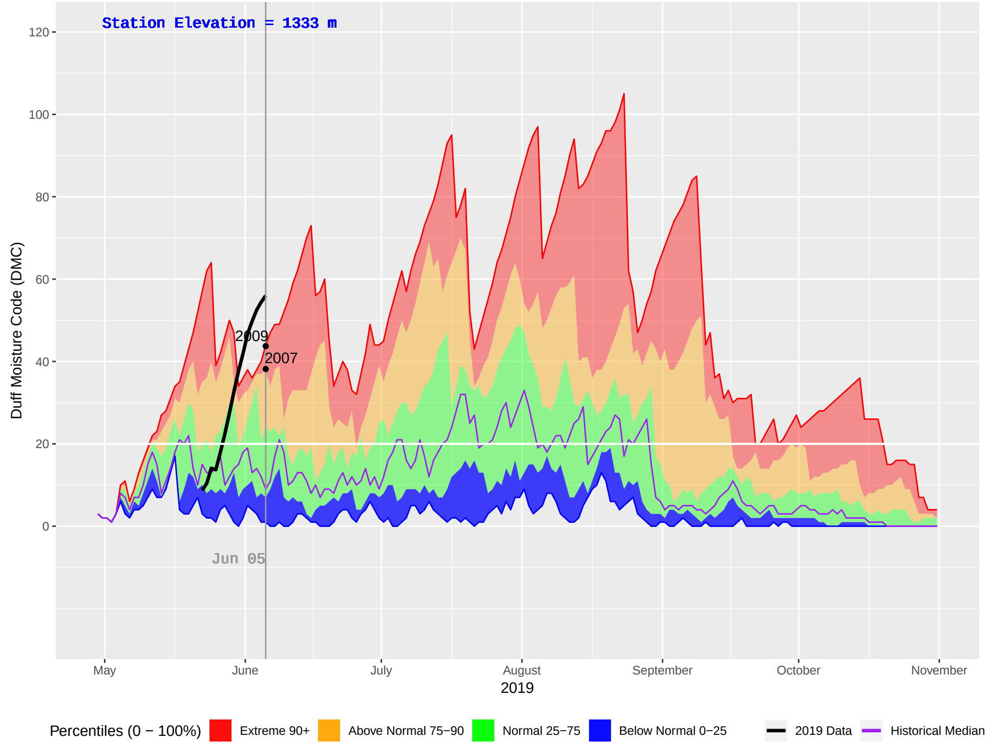
GOLDSTREAM 2 (919) : Historical (2005–2018), Current (2019) Daily Duff Moisture Code (DMC)
