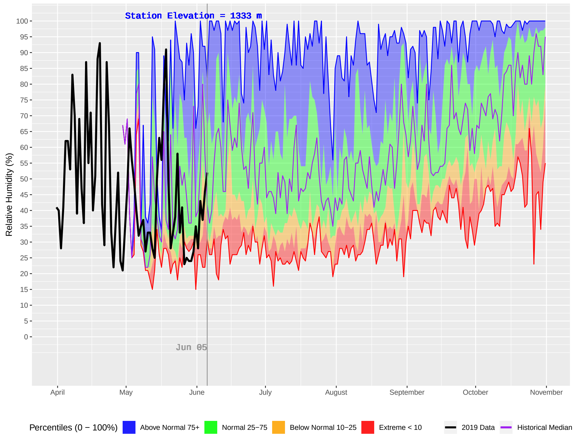
GOLDSTREAM 2 (919) : Historical (2005–2018) and Current (2019) Daily Relative Humidity
