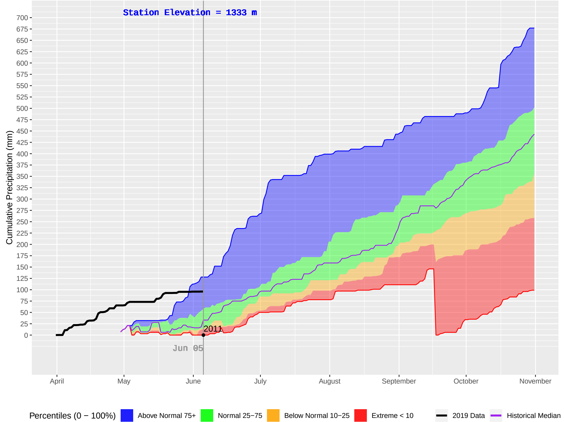
GOLDSTREAM 2 (919) : Historical (2005–2018), Current (2019) Daily Cumulative Precipitation
