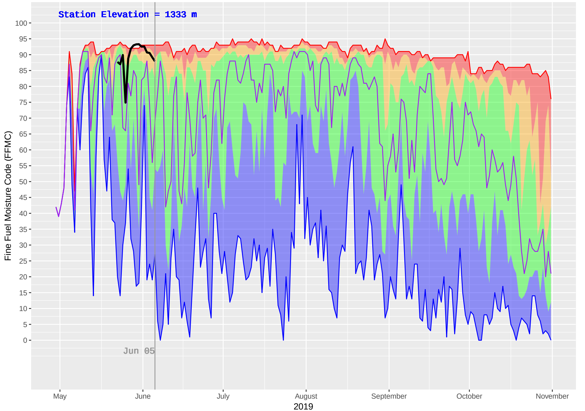
GOLDSTREAM 2 (919) : Historical (2005–2018) and Current (2019) Daily Fine Fuel Moisture Code (FFMC)
