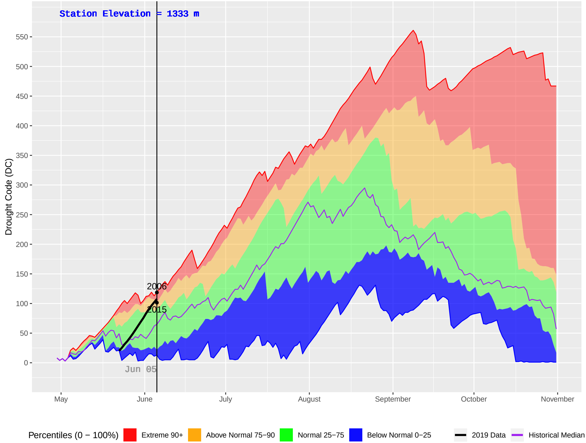
GOLDSTREAM 2 (919) : Historical (2005–2018) and Current (2019) Daily Drought Code (DC)
